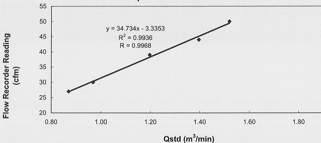
Sampler 1177 Calibration Curve
