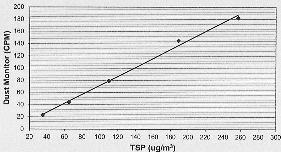
Calibration of Dust Monitor (ET/EA/001/14)
